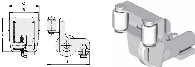
ART. 2021 A 117 B 100 C 110 L 147
