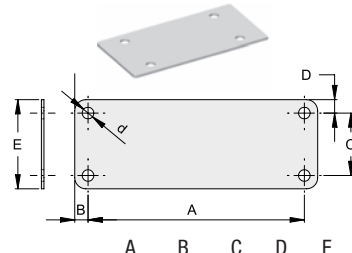
ART. 2050 A 200 B 50 C 100 D 25 E 150 d 18
